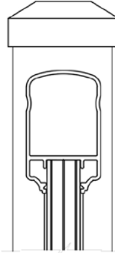
2-Rail System
