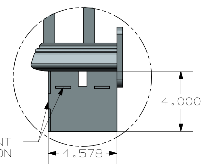
DETAIL J SCALE 1:4
